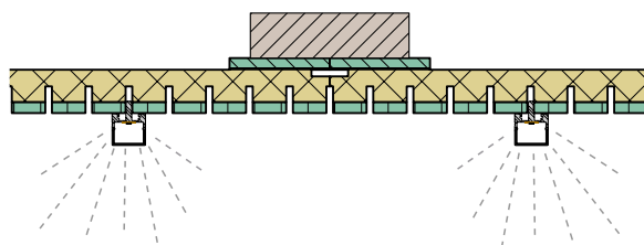
Clip-on installation:
