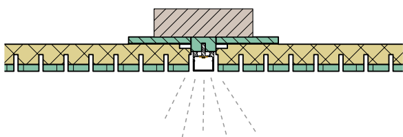
Flush installation:
